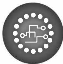
Configuration Management
